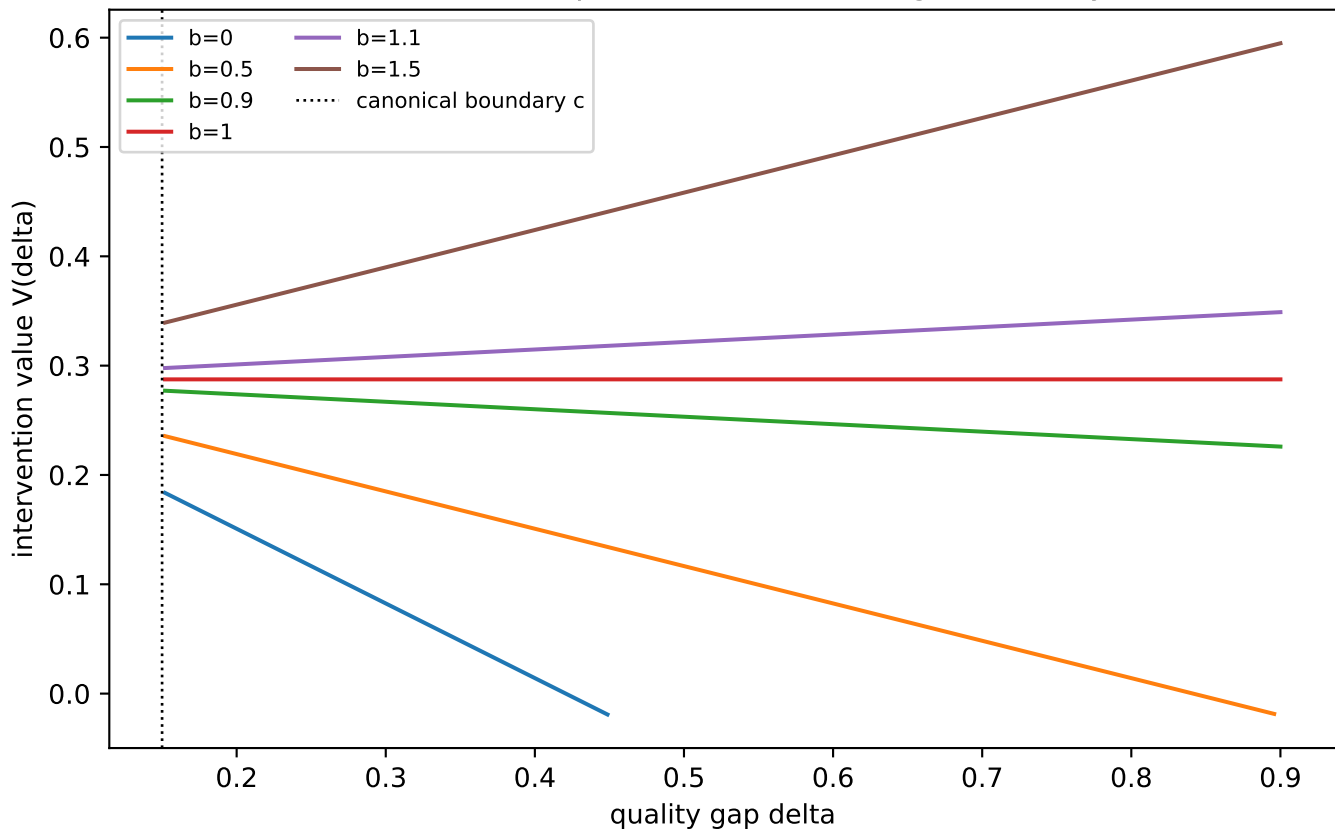
M0.1 linear response: switchable segments only
