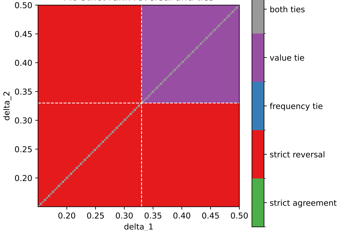
M0 strict rank reversal and ties
