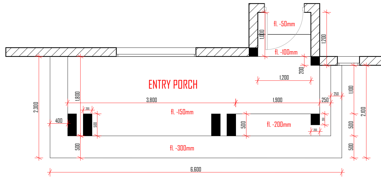
Floor Plan
