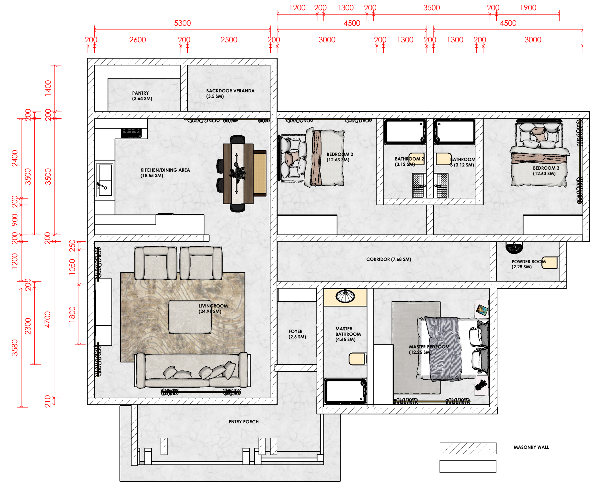
FURNITURE PLAN
