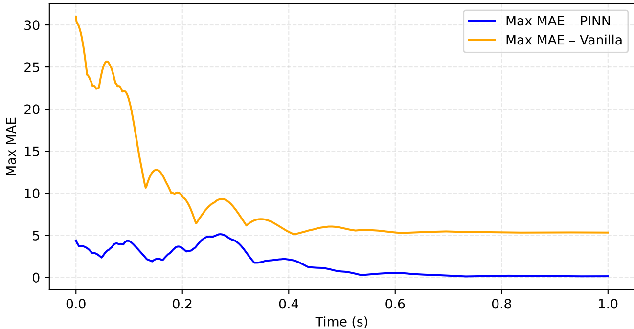
Max MAE over Time
