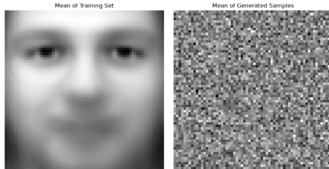
Fig. 3.4: Ablation Study Results on Olivetti Faces
