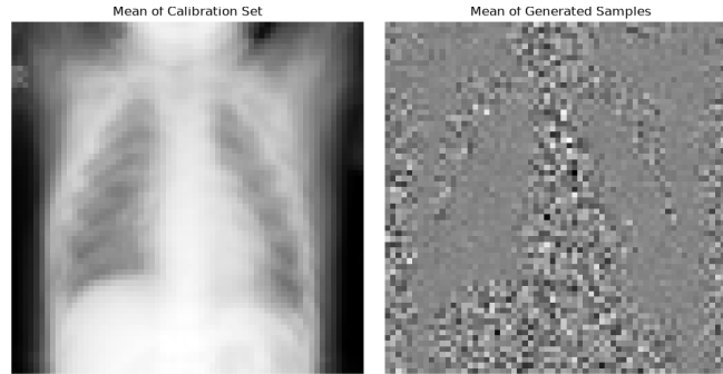
Fig. 3.2: Results on Chest X-Ray Images (Pneumonia)
