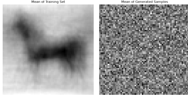
Fig. 5.6: Ablation Study Results on Weizmann Horse Database
