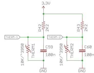
Thermistors (optional)
