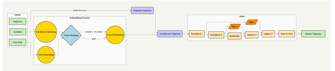
Figure 5.3: U-Net Implementation
