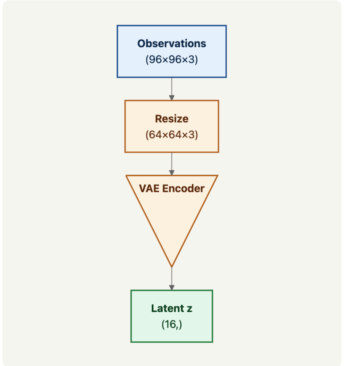
Figure A.1: VAE Pipeline
