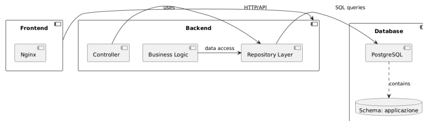
Figure 2: Diagramma componenti database.
