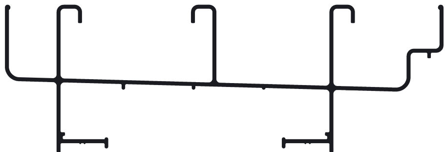
AR5-1055 Marco 3 guías 0,949 kg/m
