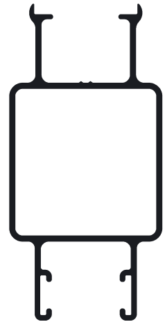
AR5-1053 Jamba reforzada 0,608 kg/m
