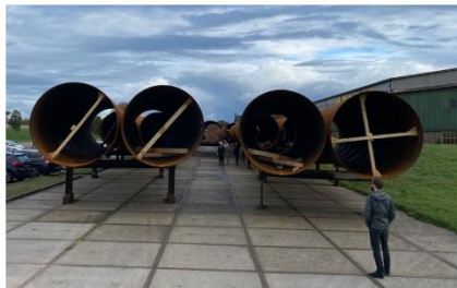
All steel tubes (Ø2.5m) arrived at assembly site.
