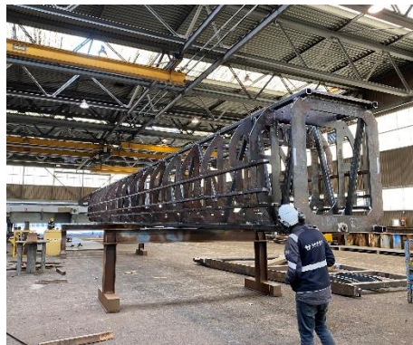
Assembly jig for pipe sections
