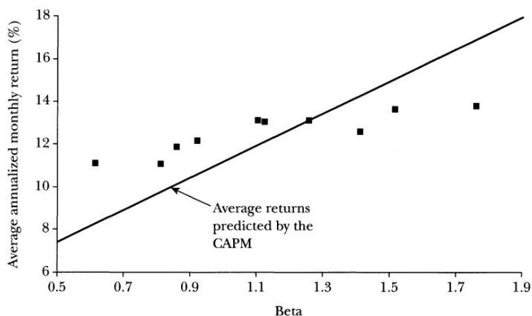
Figure 1.18: The empirical security market line is too flat. Average annualized monthly returns of ten value-weight portfolios sorted on prior beta, 1928–2003, against the average returns predicted by the CAPM. Low-beta portfolios earn more, and high-beta portfolios less, than the CAPM implies. Source: Fama and French (2004).
