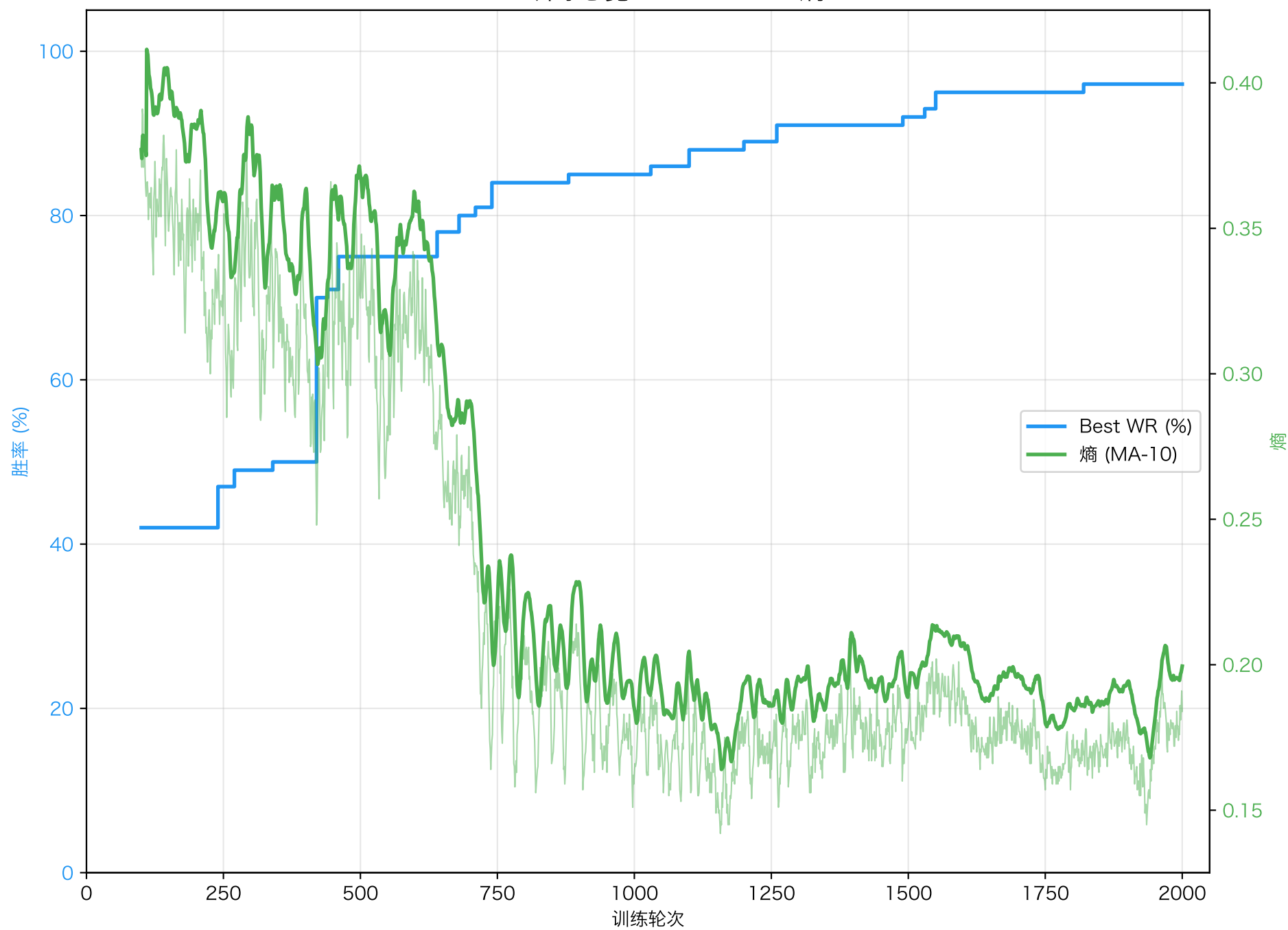
v49 训练总览: Best WR vs 熵
