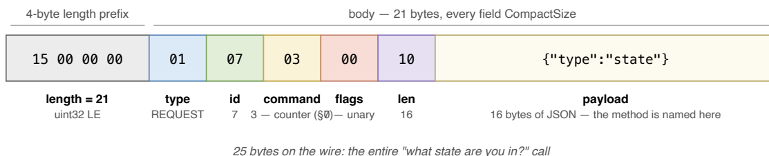
FIGURE 2. A complete unary request frame, byte by byte.
