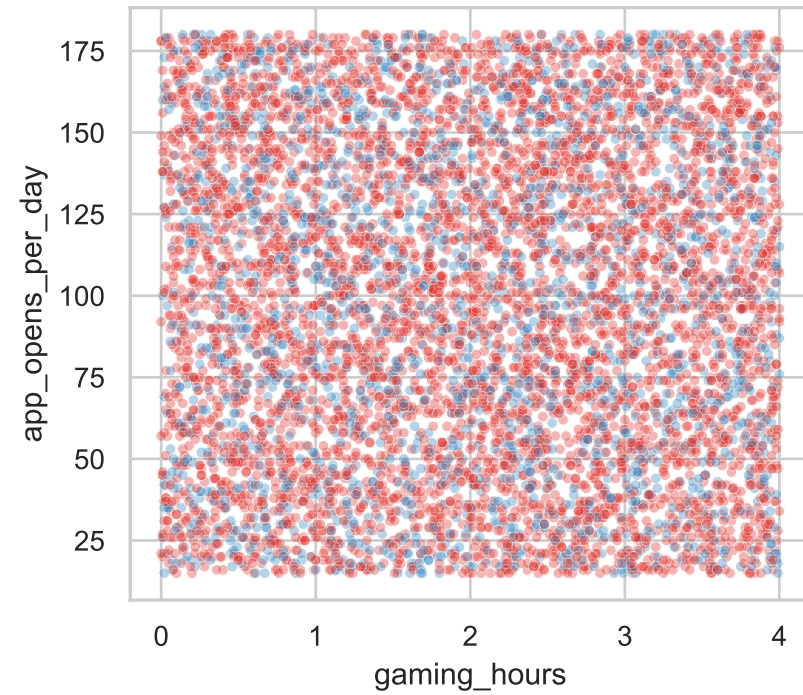
gaming hours vs. app opens per day
