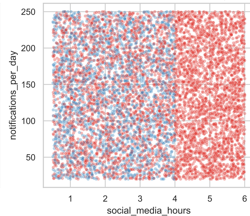
social media hours vs. notifications per day
