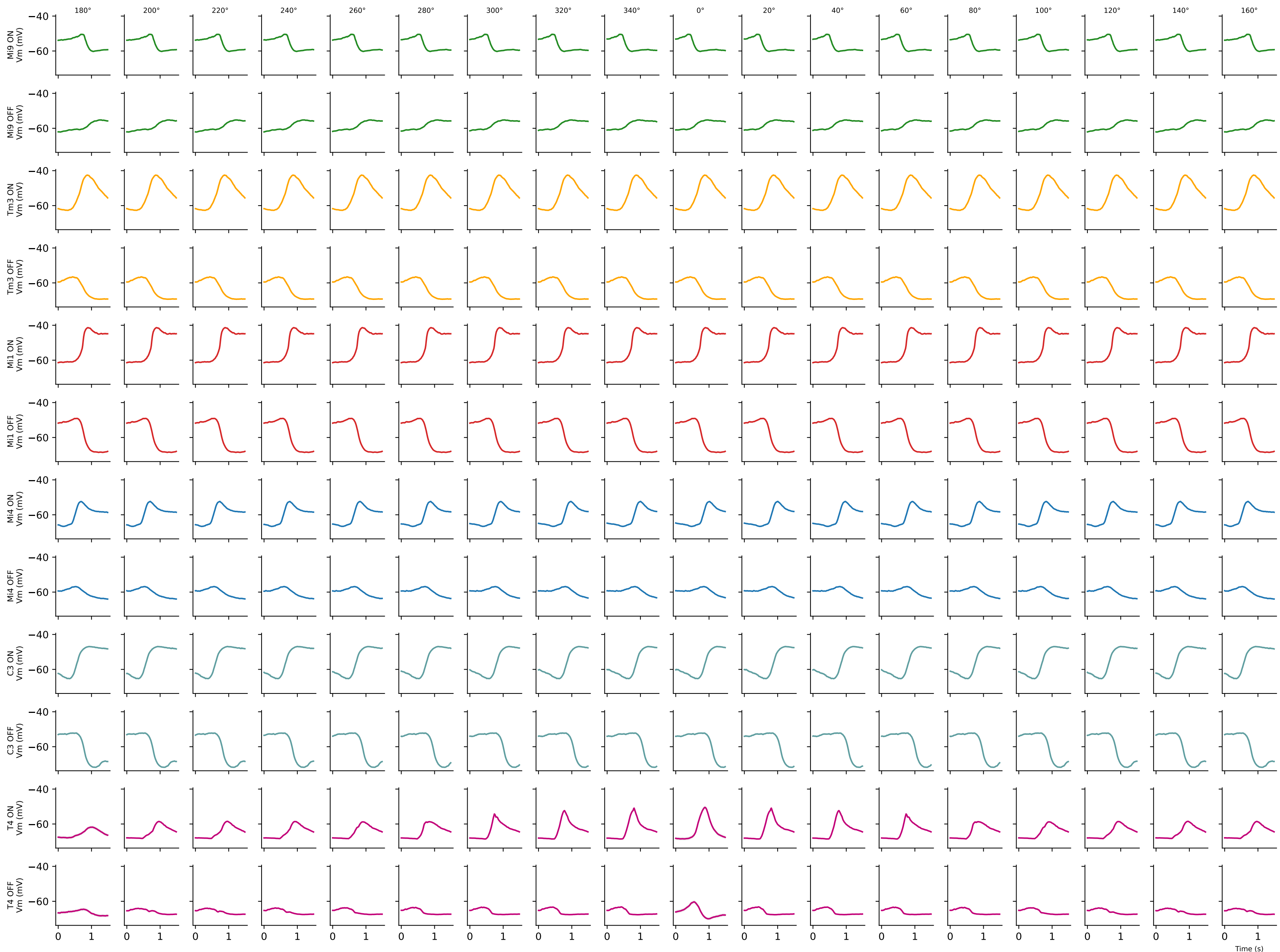
Six-neuron Vm (30°/s edges): presynaptic measured; T4 measured at PD/ND, model elsewhere
