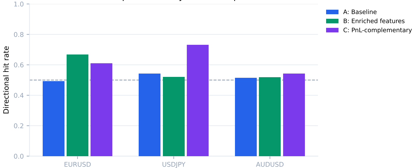
Test-split hit rate by mode and pair
