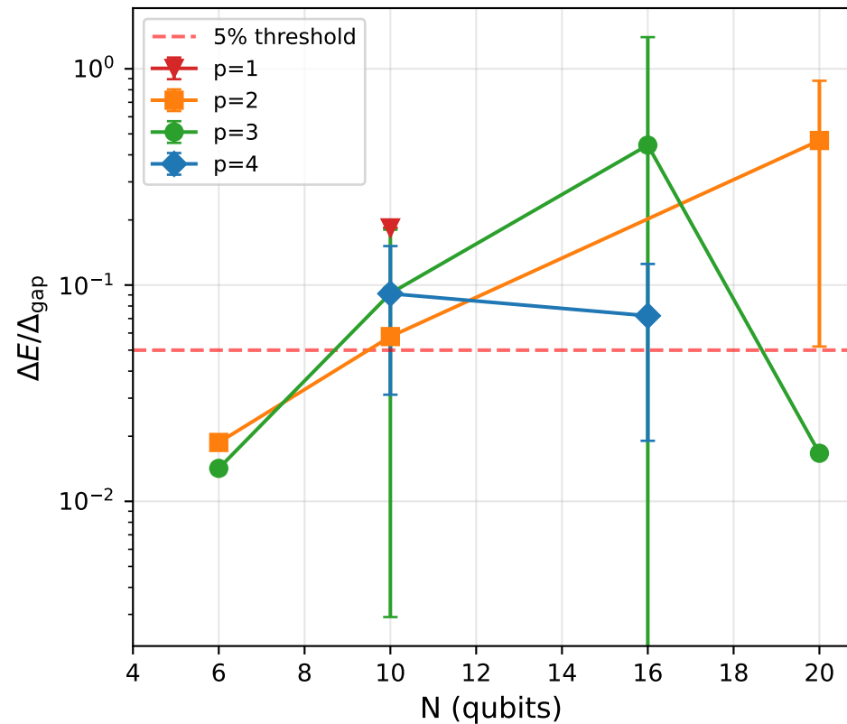
\Delta E/\Delta_{\text{gap}} vs System Size
