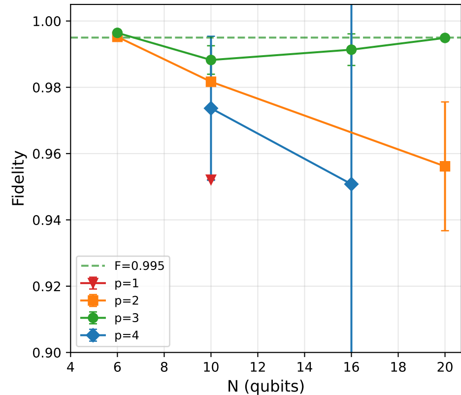
Fidelity vs System Size
