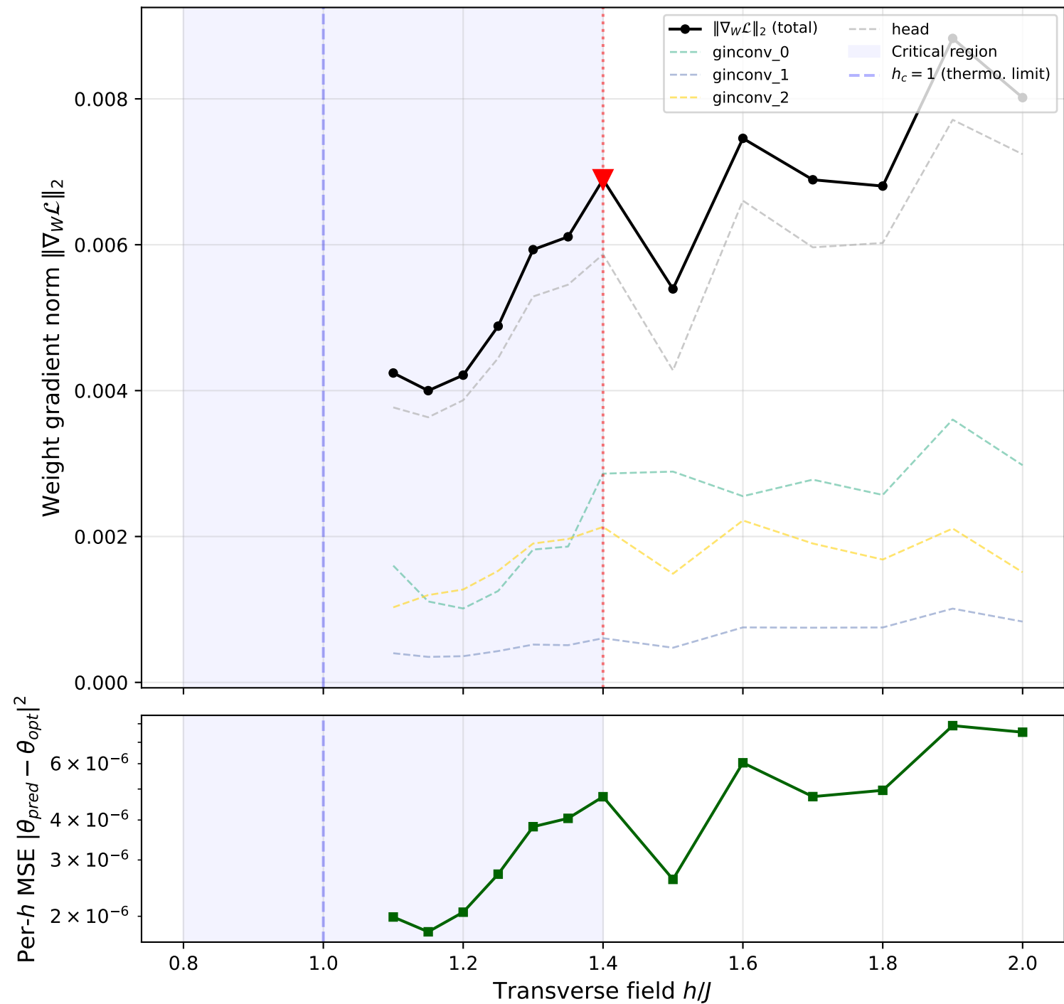
Phase Transition Signature in MPNN Weight Space (N=10, 1D TFIM, GINConv h=128 , seed=43 — Hernandez et al. 2025)
