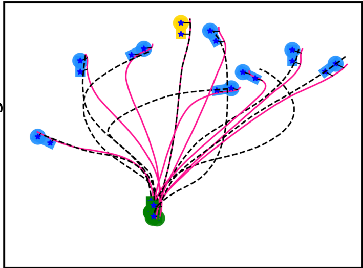
Laplacian Editing
