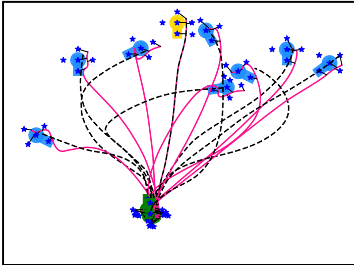
Laplacian Editing
