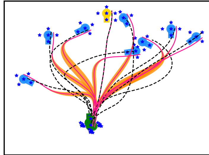
Gaussian Process Transportation
