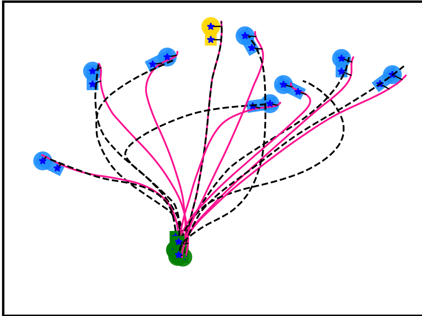
Laplacian Editing
