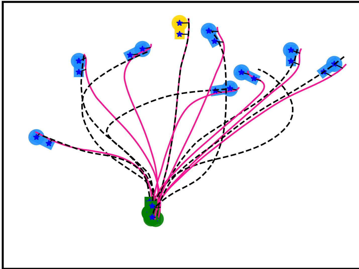
Laplacian Editing
