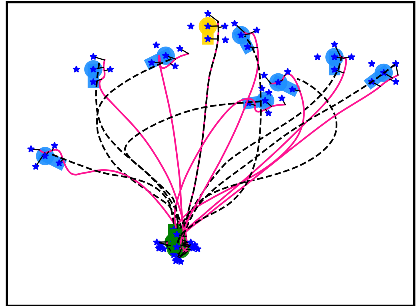
Laplacian Editing
