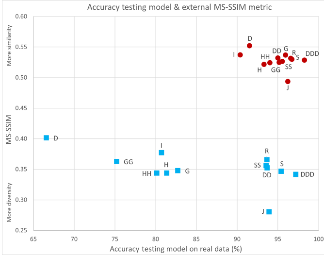
Fig. 18: Accuracy of model testing and external MS-SSIM metric. The red circles indicate datasets with real and augmented data, and turquoise squares are entirely augmented datasets. The codes are described in Table VIII.
