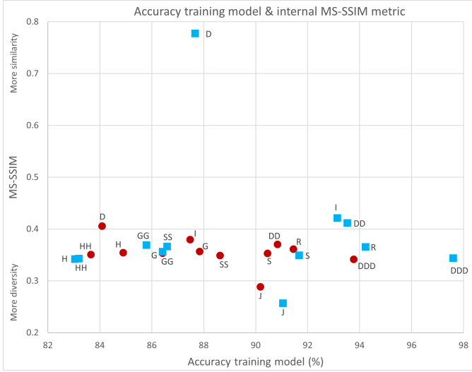
Fig. 14: Zooming at figure of model training accuracy and internal MS-SSIM metric. The green shape indicates real dataset with 62.8% of accuracy (which is not visible because the segment with accuracy \geq 82\% is displayed), red circles indicate datasets with real and augmented data, and turquoise squares are entirely augmented datasets. The codes are described in table VIII.
