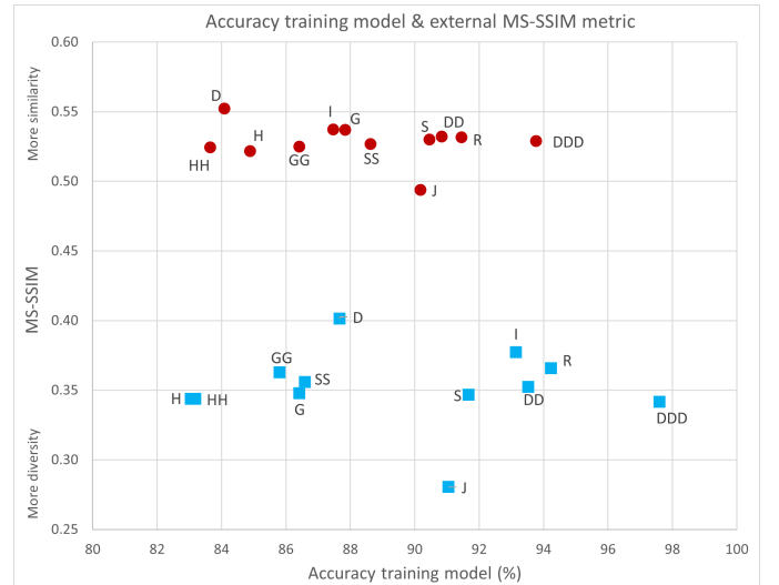
Fig. 17: Zooming at figure of model training accuracy and external MS-SSIM metric. The green shape indicates real dataset with 62.8% of accuracy (which is not visible because the segment with accuracy \geq 80\% is displayed), red circles indicate datasets with real and augmented data, and turquoise squares are entirely augmented datasets. The codes are described in table VIII.
