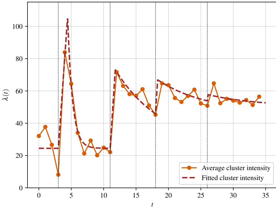
Cluster 2
