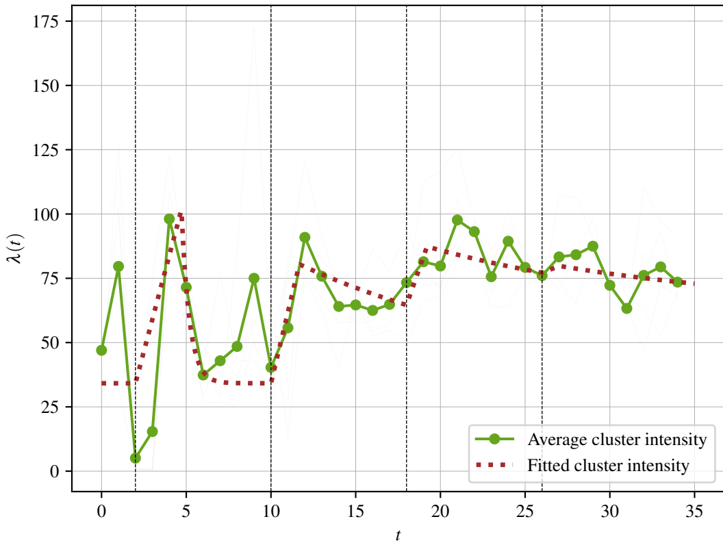
Cluster 5
