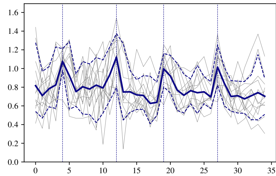
Cluster 3
