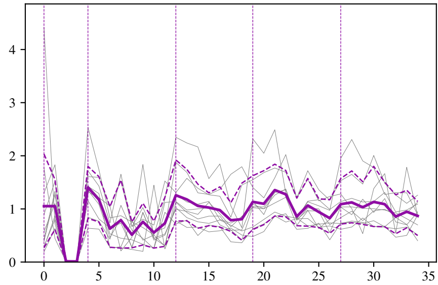
Cluster 6
