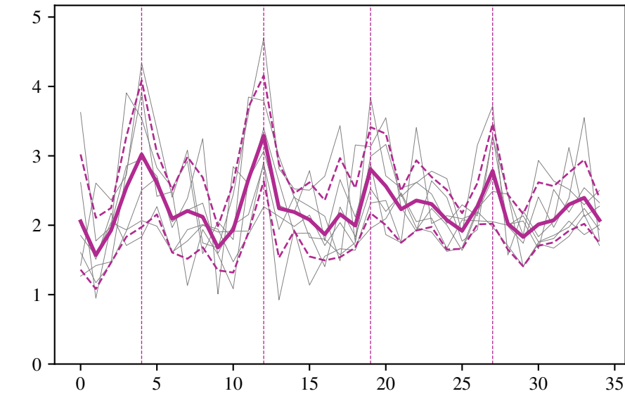
Cluster 7
