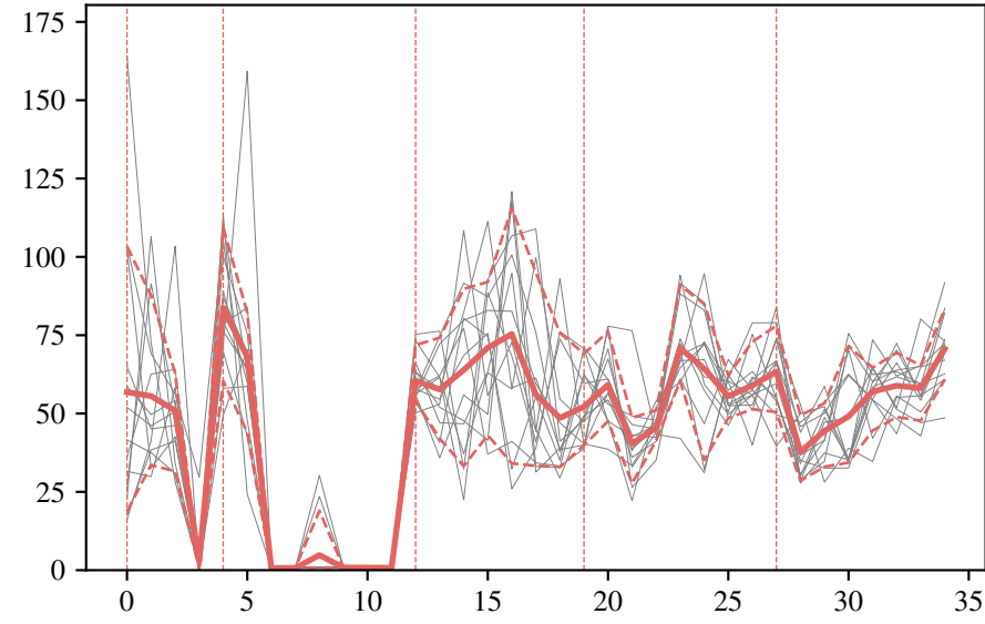
Cluster 9
