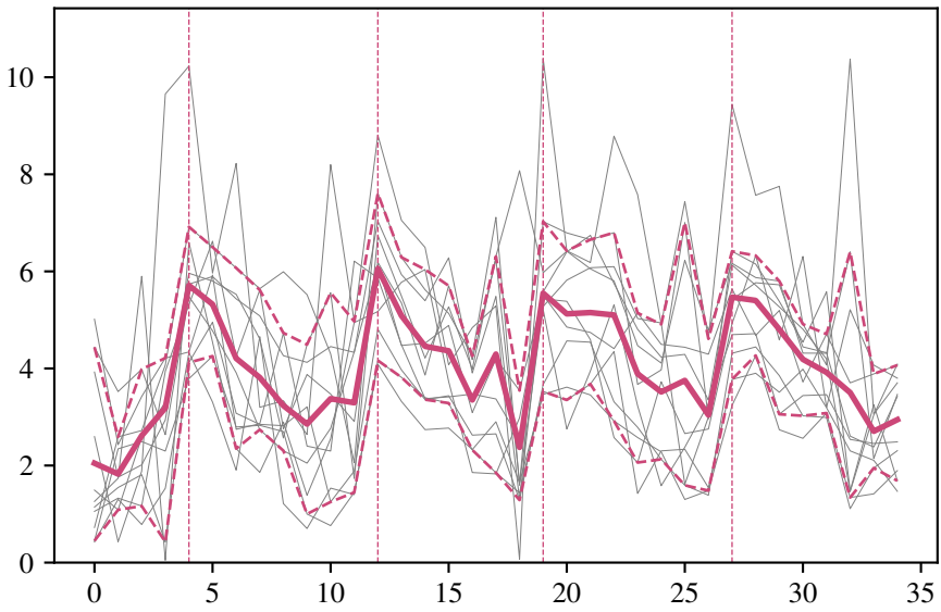
Cluster 8
