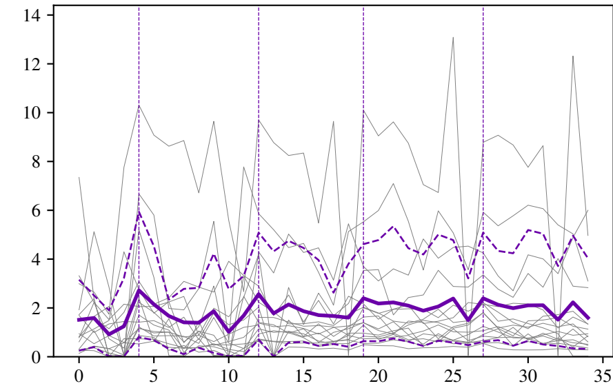
Cluster 5
