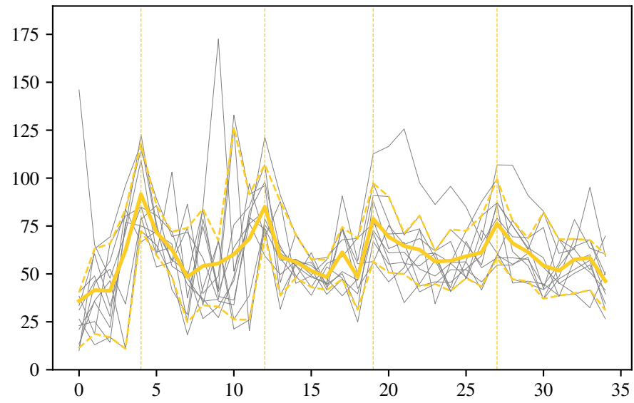
Cluster 10
