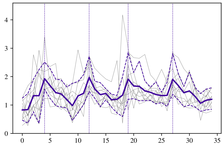
Cluster 4
