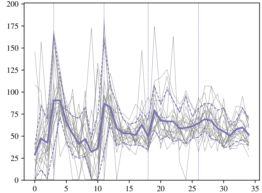
Cluster 3
