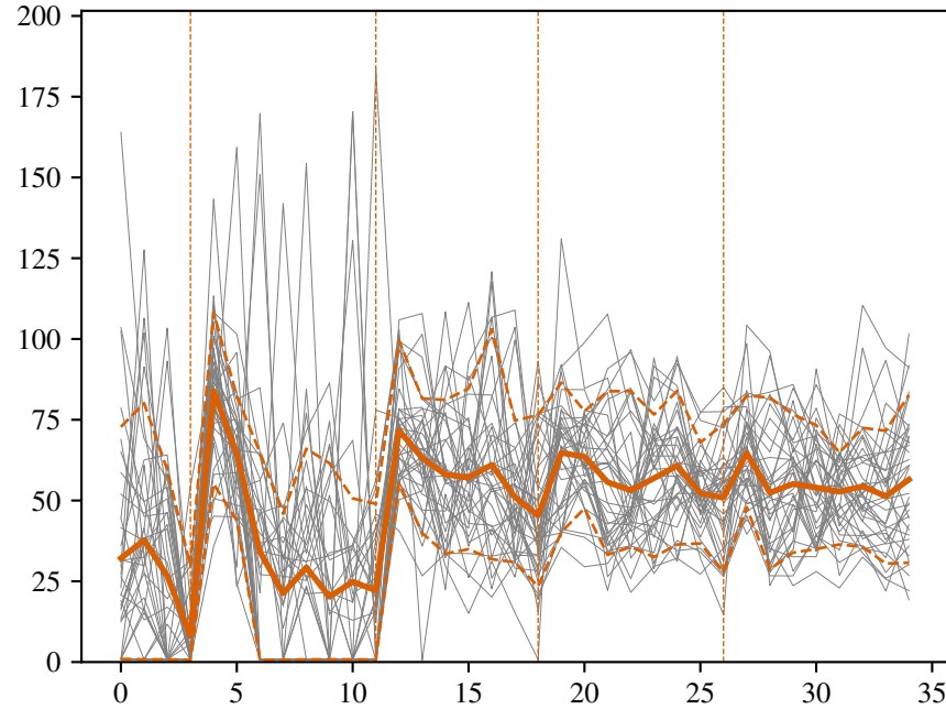
Cluster 2
