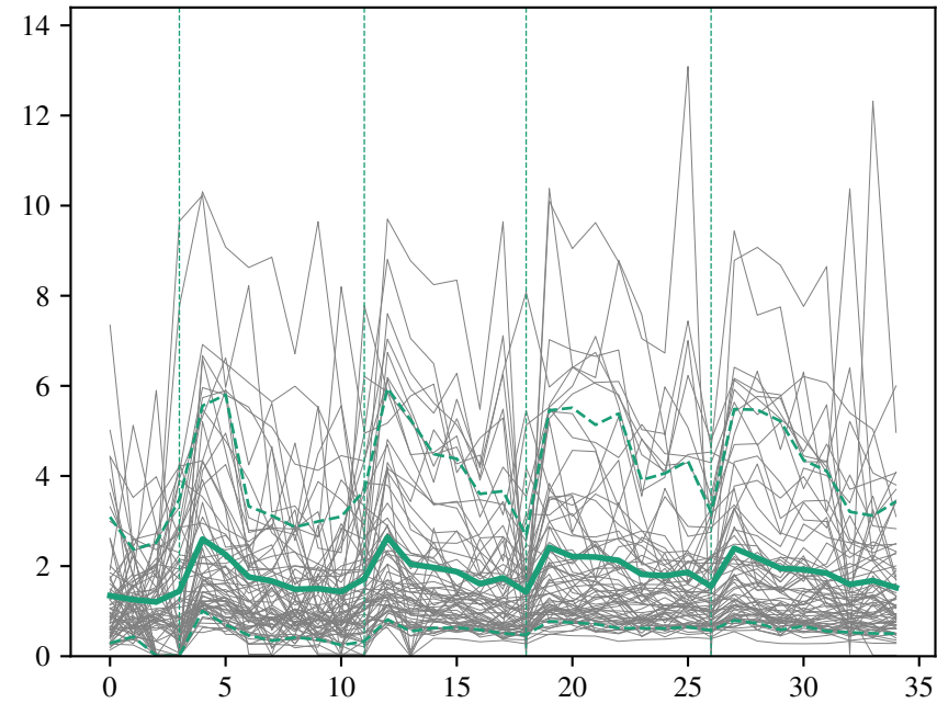
Cluster 1
