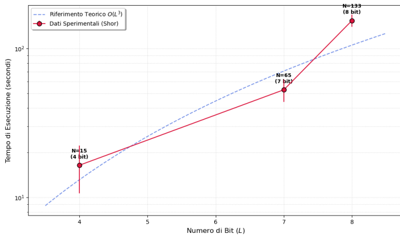
Figure 3: Execution time vs. number of bits L = \lceil \log_2 N \rceil on a semi-log scale. Are included 3 executions to estimate the error. Experiment was performed on MPS simulator backend.
