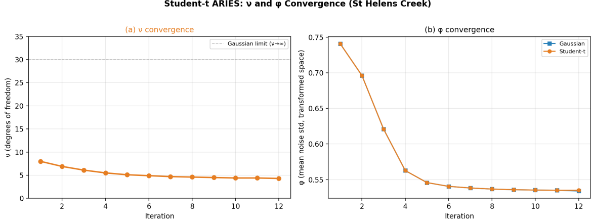
Figure 1: (a) Degrees of freedom \nu converges from 8.0 to 4.3 across 12 ARIES iterations, confirming heavy-tailed residuals. The Gaussian limit ( \nu \rightarrow \infty , dashed line) is strongly rejected. (b) Mean observation noise \phi converges identically under both likelihoods, confirming that the latent weights \lambda_i absorb outlier variance rather than inflating the baseline noise estimate.
