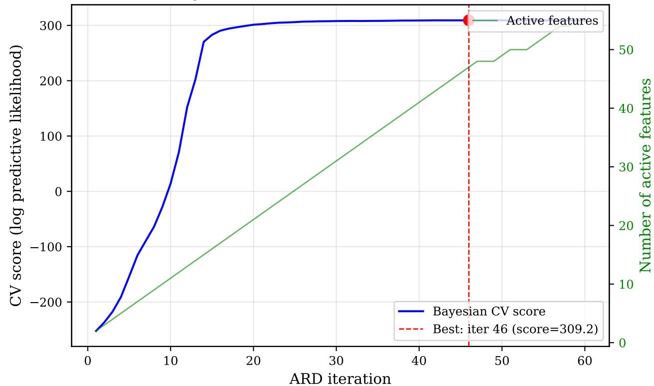
Ishigami Function: ARD-CV Model Selection
