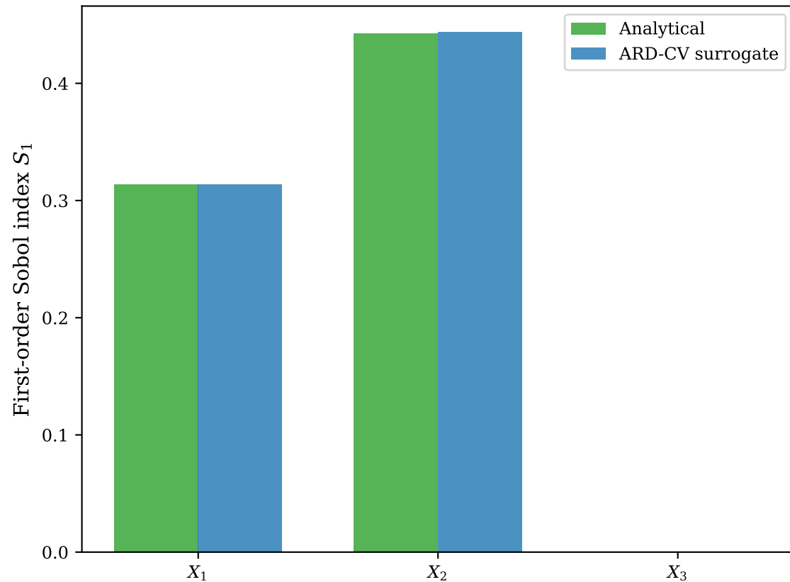
Sensitivity Recovery
