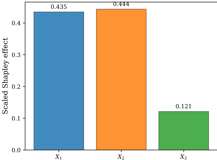
Ishigami: Shapley Effects (ARD-CV surrogate)
