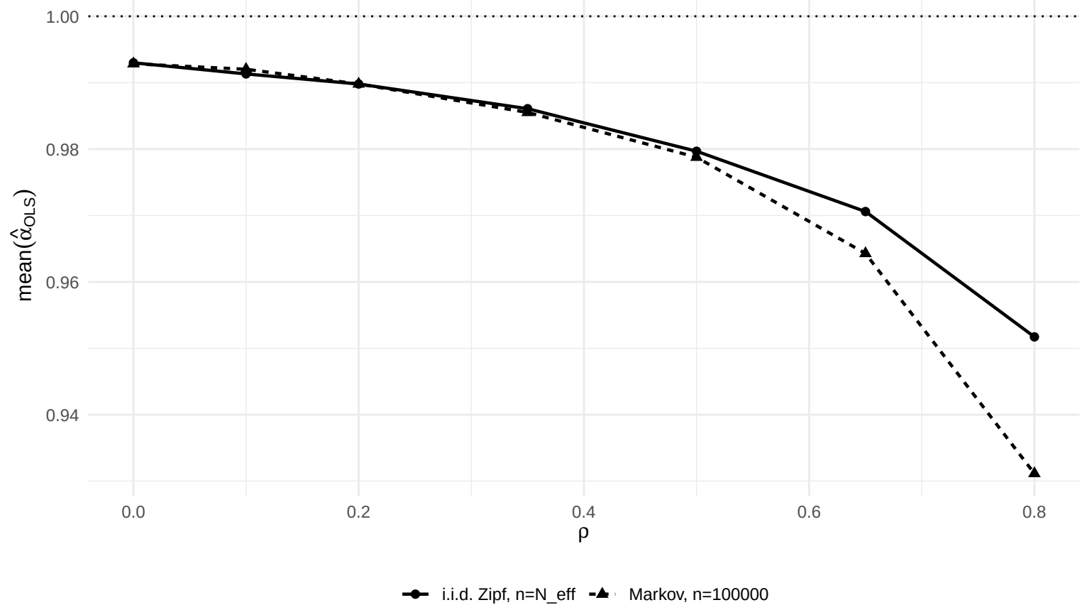
Finite-sample exponent shift under increasing dependence
