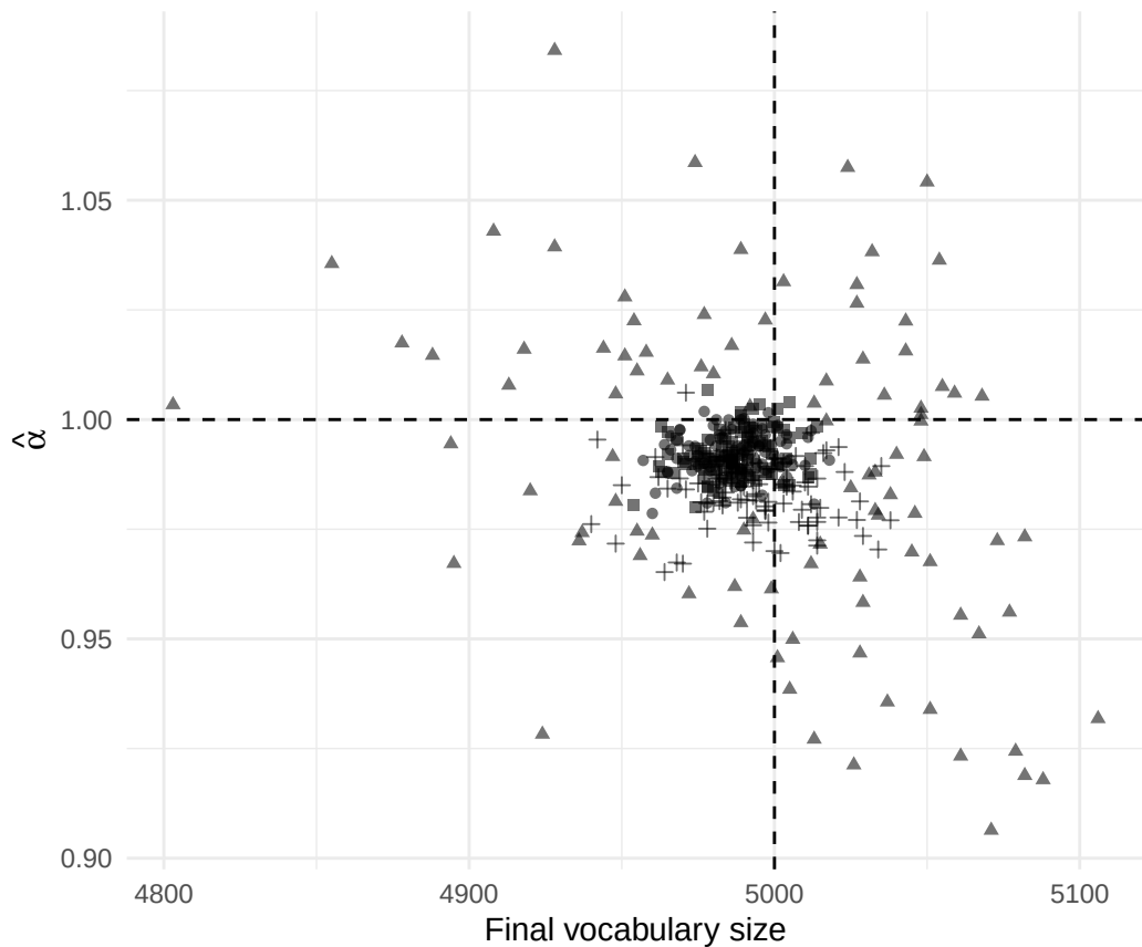
A. Joint matching on exponent and final vocabulary
