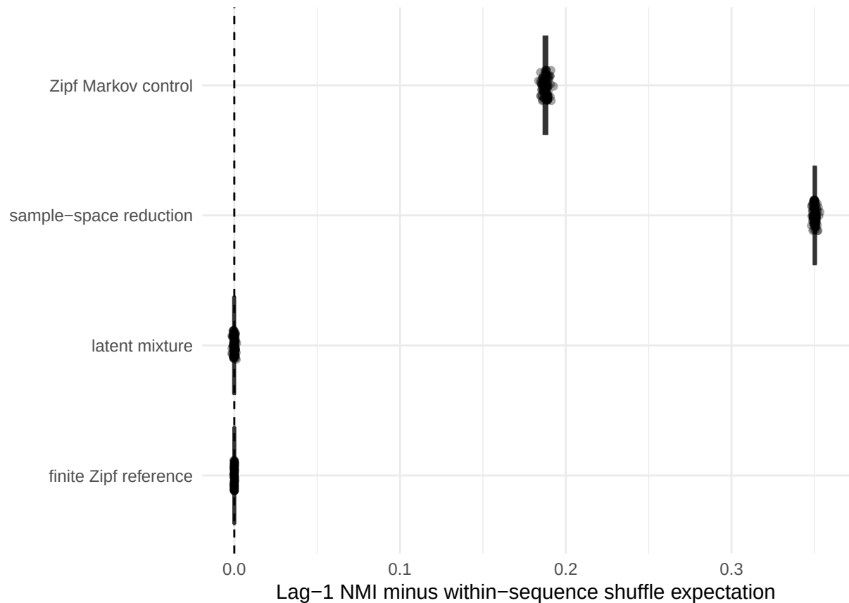
B. Sequence information persists after joint matching
