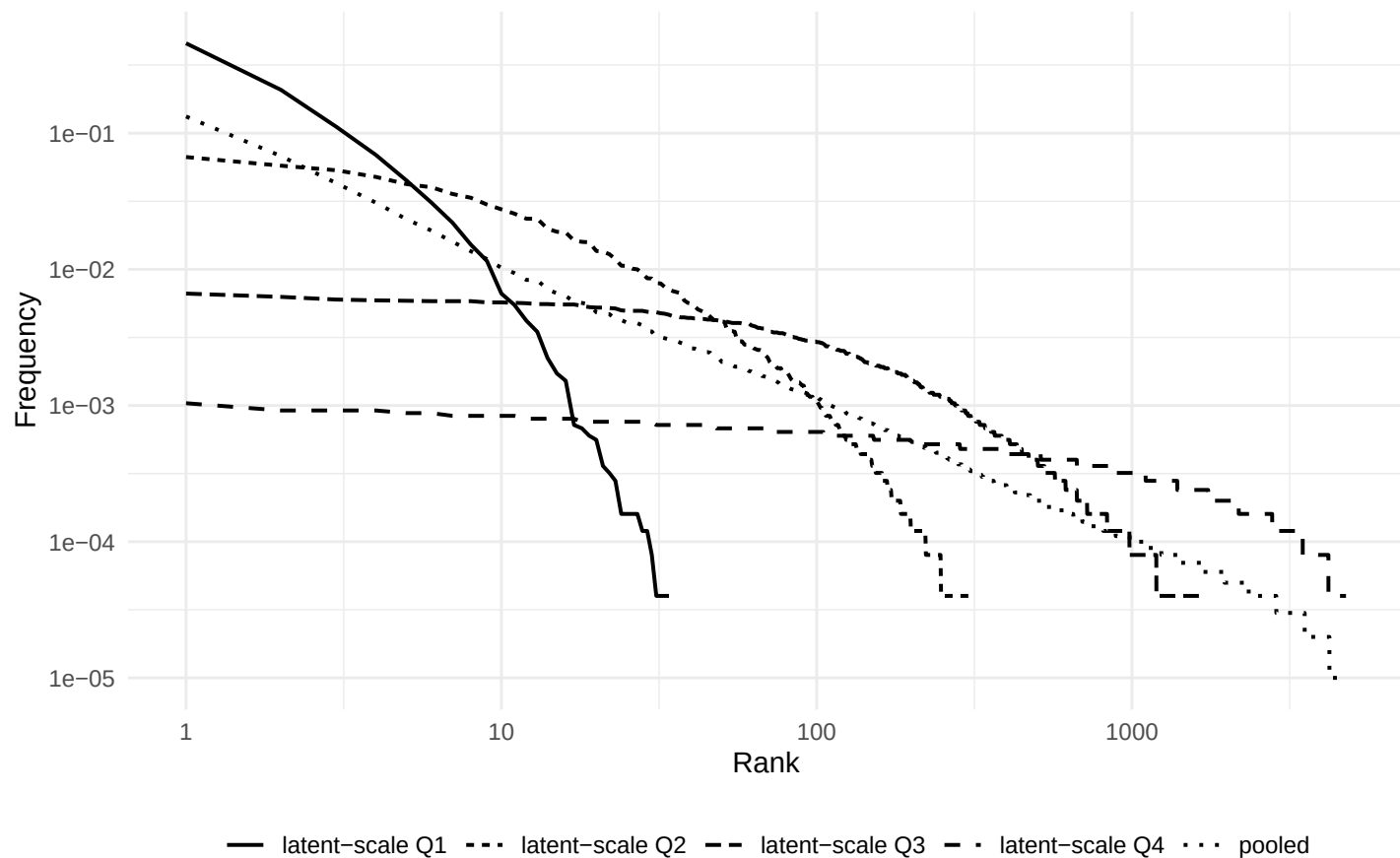
Pooling can create scaling absent within latent regimes
