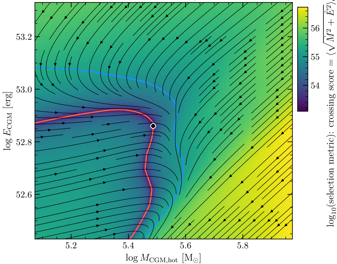
a' metric map at t = 0.16 Gyr ( z = 21.43 redshift)
