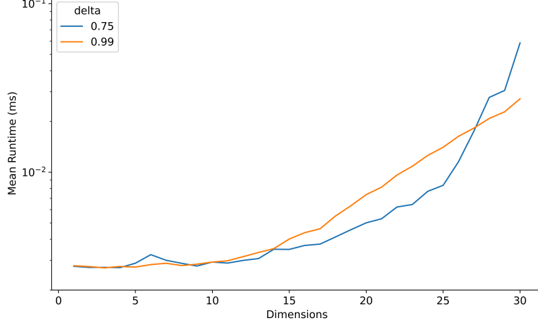
FIGURE 1. Run-time in milliseconds plotted against the dimensionality of the basis for delta values of 0.75 and 0.99.
