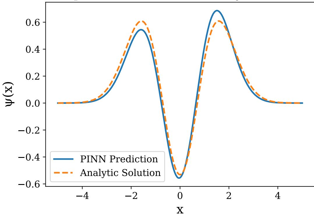
Comparison of PINN and Analytic Solution
