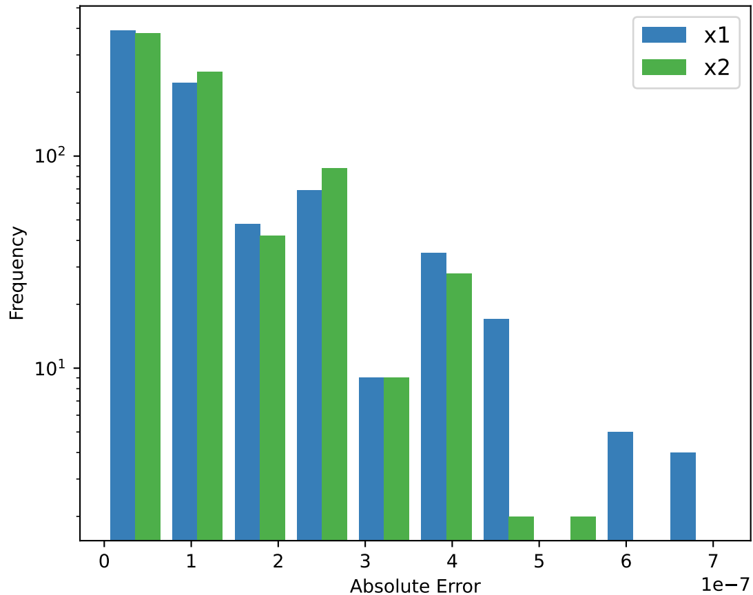
Invertibility Errors (Max: 7.15e-07)
