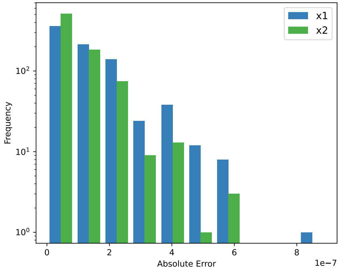
Invertibility Errors (Max: 8.94e-07)
