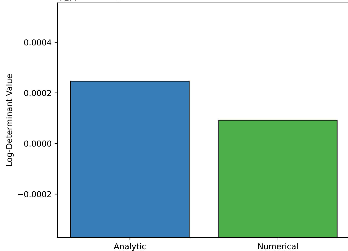
Log-Determinant Check (Error: 1.54e-04)
