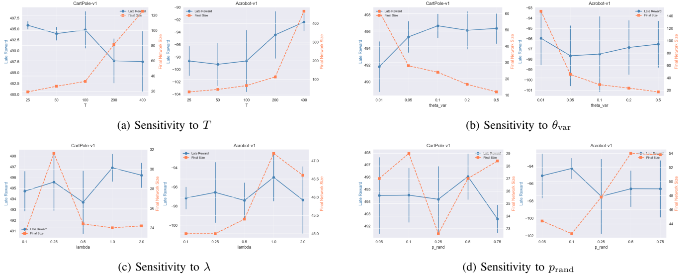
Fig. A.1: One-factor-at-a-time sensitivity curves for the four primary SPM hyperparameters on CartPole-v1 and Acrobot-v1. Error bars indicate across-seed variability. Across the tested parameters, T exhibits the clearest task dependence, while \theta_{\text{var}} most directly controls final network compactness.
