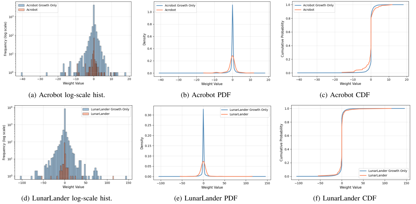
Fig. A.2: Additional weight distributions for the growth-only and SMGrNN configurations on Acrobot-v1 and LunarLander-v3.
