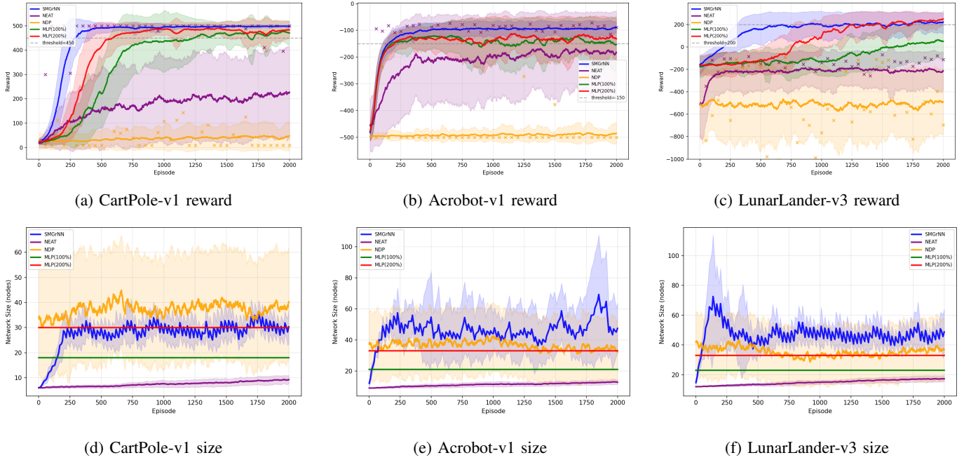
Fig. 3: Comparison with fixed-topology and dynamic-topology baselines. Top row: reward evolution for SMGrNN, MLP baselines, NEAT, and NDP. Solid curves show smoothed mean returns over 10 seeds for the gradient-trained models and the smoothed evaluation trajectory for the evolutionary baselines. Shaded regions indicate across-seed variability, and dashed horizontal lines mark task-specific reward thresholds. For NEAT and NDP, cross markers indicate the performance of the best individual selected in each evolutionary generation. Bottom row: network-size evolution and final network sizes. SMGrNN expands to task-dependent graph sizes; NEAT exhibits approximately linear structural growth; NDP often produces larger and more variable structures. MLP baselines have fixed sizes by construction.
