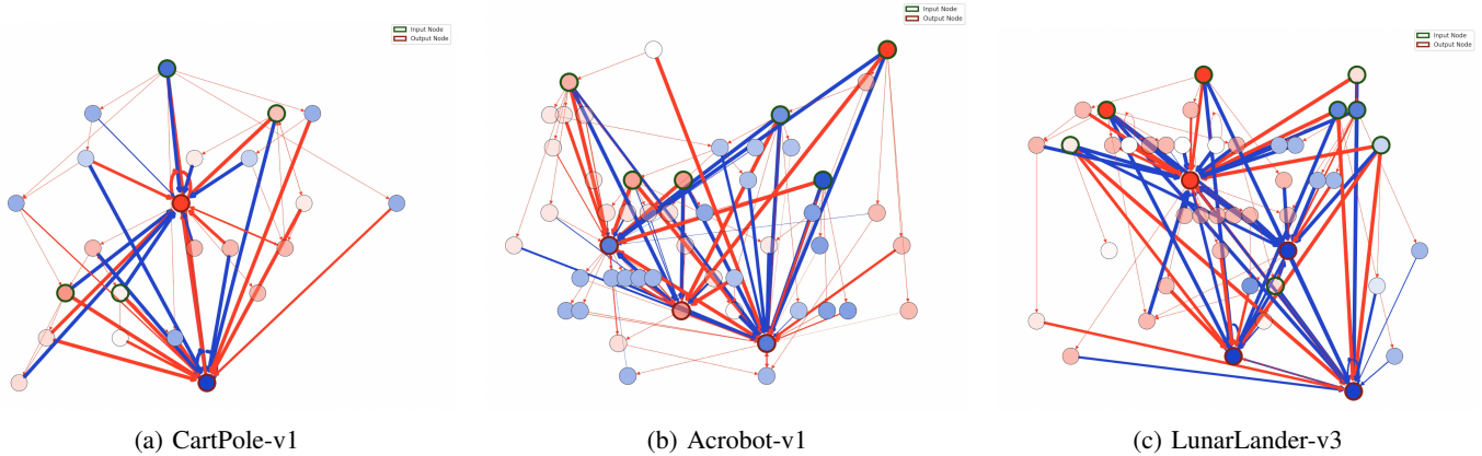
Fig. 8: Representative final SMGrNN topologies after training on CartPole-v1, Acrobot-v1, and LunarLander-v3. Input nodes are outlined in green and output nodes in red. Edge color and width indicate signed weight magnitude. The learned graphs are sparse, directed, and non-layered, illustrating how local structural plasticity produces task-dependent topologies that differ substantially from a fixed multilayer perceptron.
