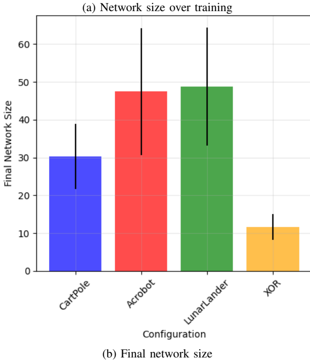
Fig. 7: Scaling of SMGrNN capacity with task difficulty. Left: hidden-node trajectories; right: final hidden-node counts.
