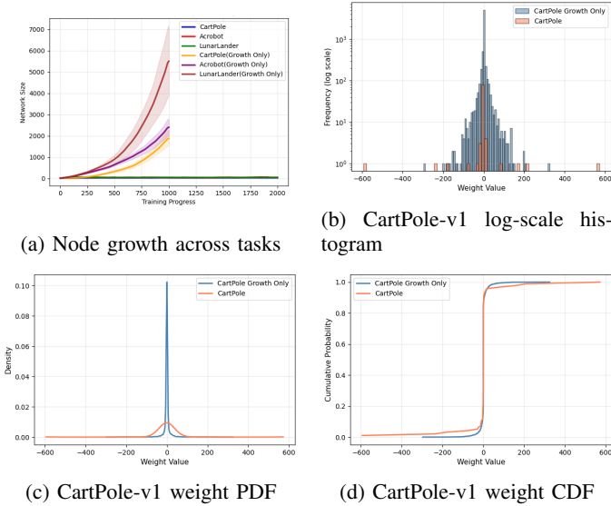
Fig. 5: Growth-only variant vs. SMGrNN. Panel (a) shows the number of nodes over training for all environments. Panels (b)–(d) show final weight distributions on CartPole-v1: log-scale histogram, probability density function (PDF), and cumulative distribution function (CDF).
