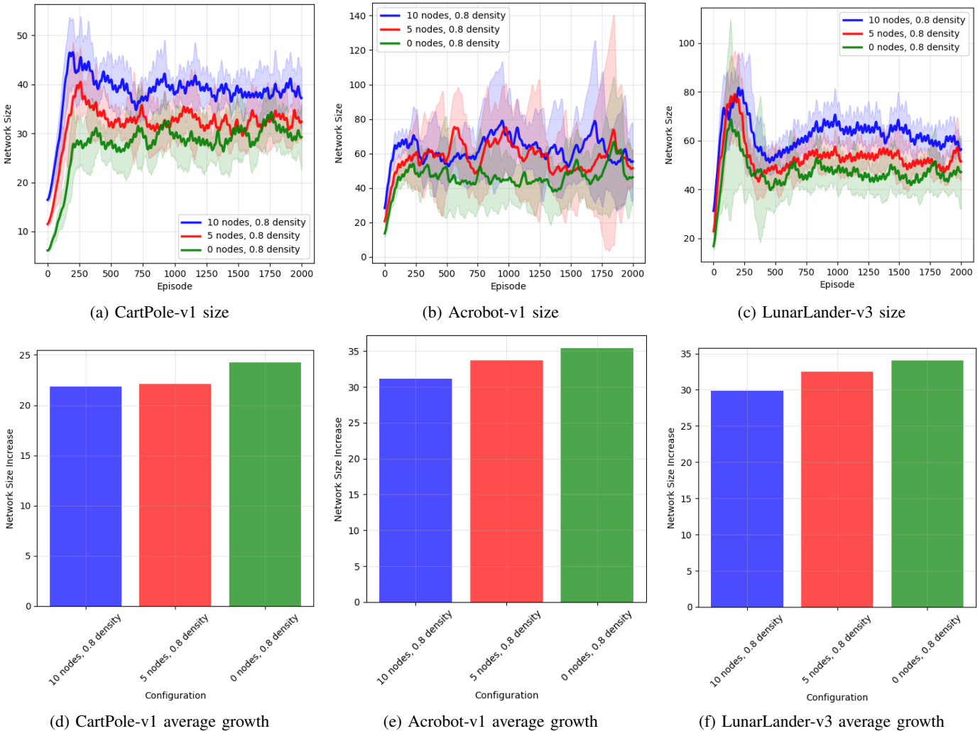
Fig. 6: Sensitivity to initial topology. Each panel averages over 10 runs with initial hidden-node counts 0, 5, and 10 under identical SPM hyperparameters. Top row: number of hidden nodes over training; bottom row: average growth per episode.
