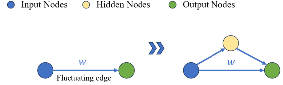
Fig. 2: Relay-node insertion on an unstable edge in a minimal network. Left: a single input–output connection whose update direction remains unresolved over the observation window and whose normalized fluctuation satisfies Eq. (4). Right: when the edge is flagged as unstable, the SPM inserts a new relay node and a two-step pathway, while retaining the original edge. The example shows a one-input, one-output network for clarity, but the same mechanism can be applied to any edge in a larger SMGrNN graph that satisfies Eq. (4).
