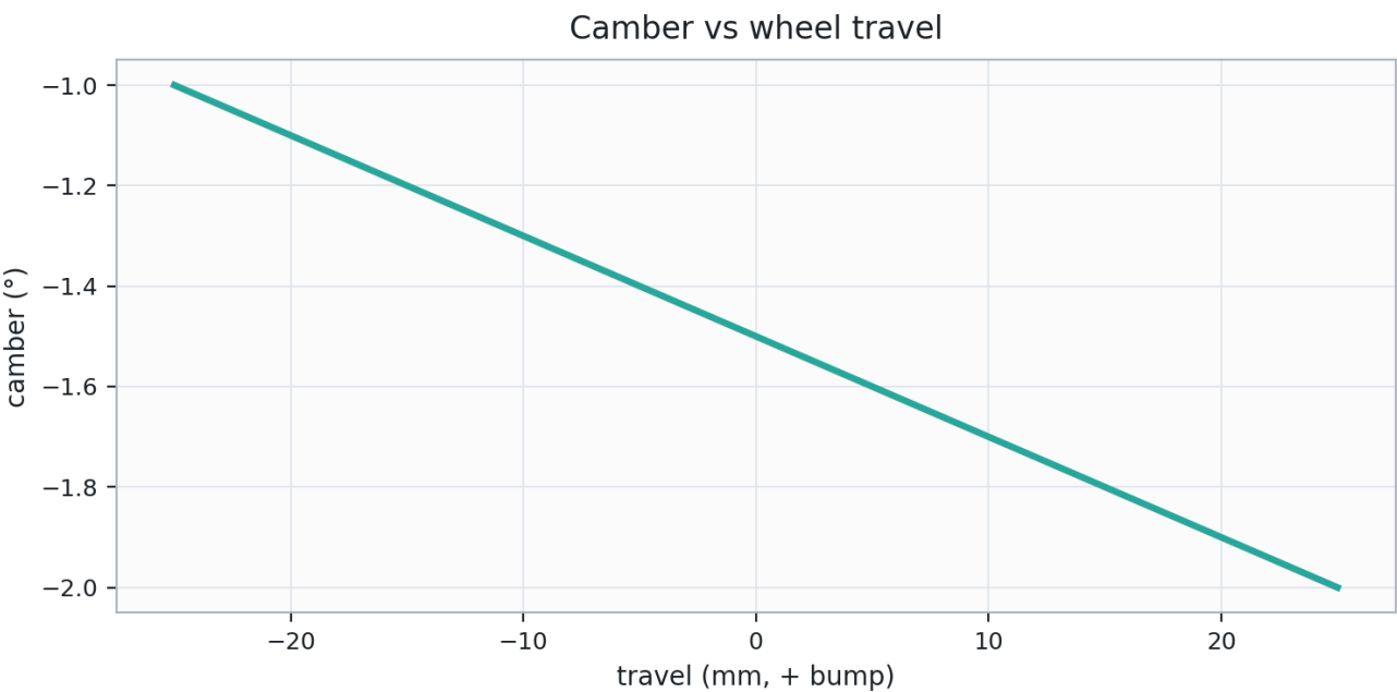
Camber vs wheel travel — camber (°) vs travel (mm, + bump) · 1 series
