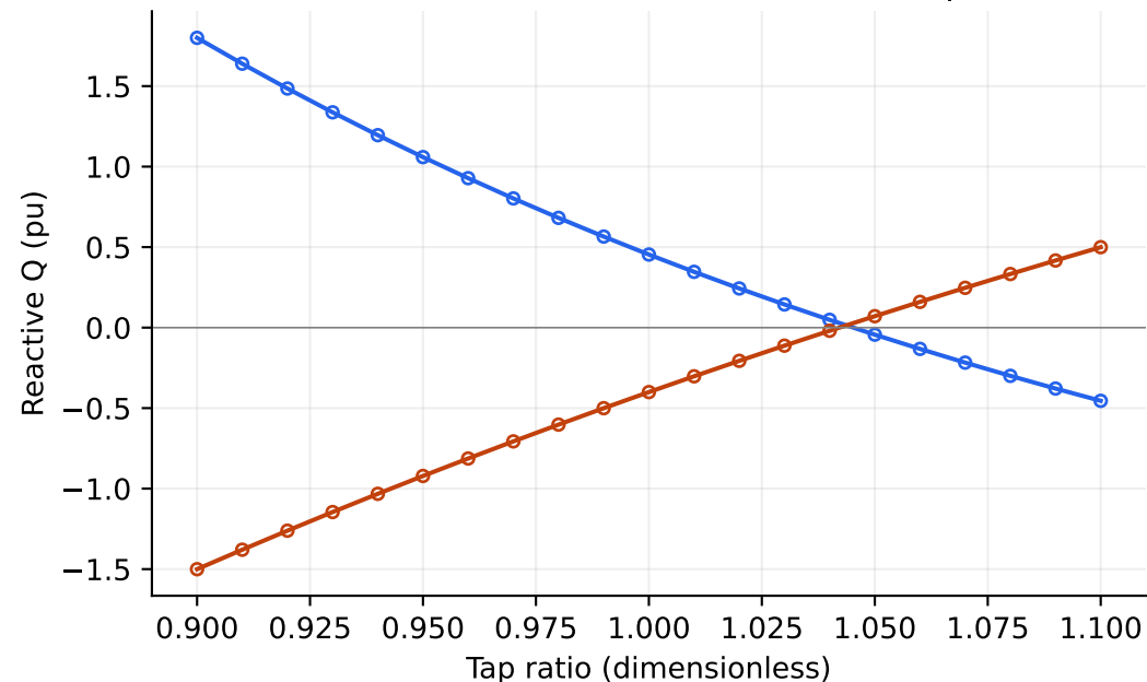
M5.3 signed phase · max error 4.0e-15 pu
