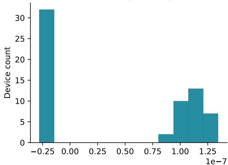
Bank susceptance (pu)
