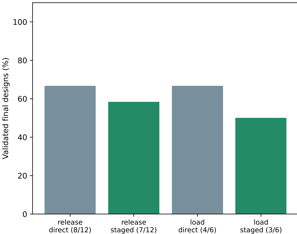
ipopt
