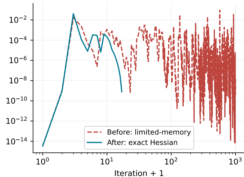
96 buses · NLP constraint violation
